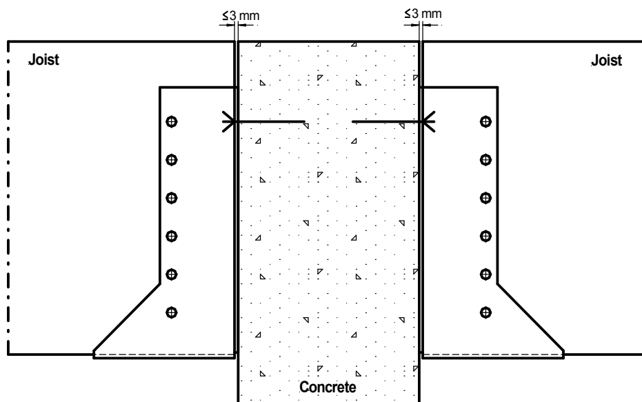
Figure A.2.4: BB joist hanger connected to concrete, lightweight concrete or steel members by bolts
