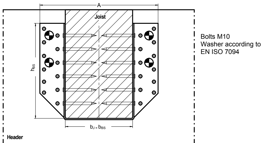
Figure A.2.3: BB joist hanger connected to concrete, lightweight concrete or steel members by bolts
